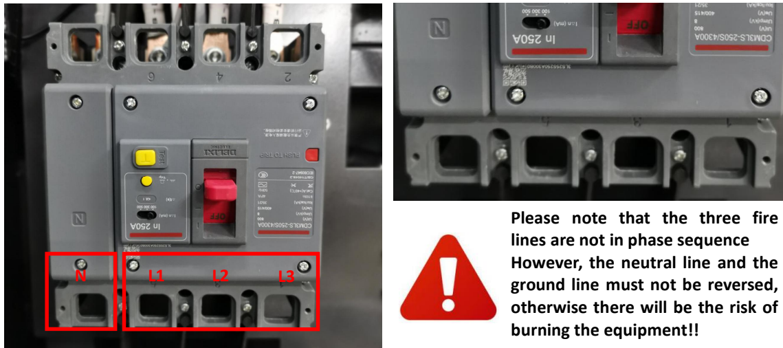
L wire and N wire connection position
