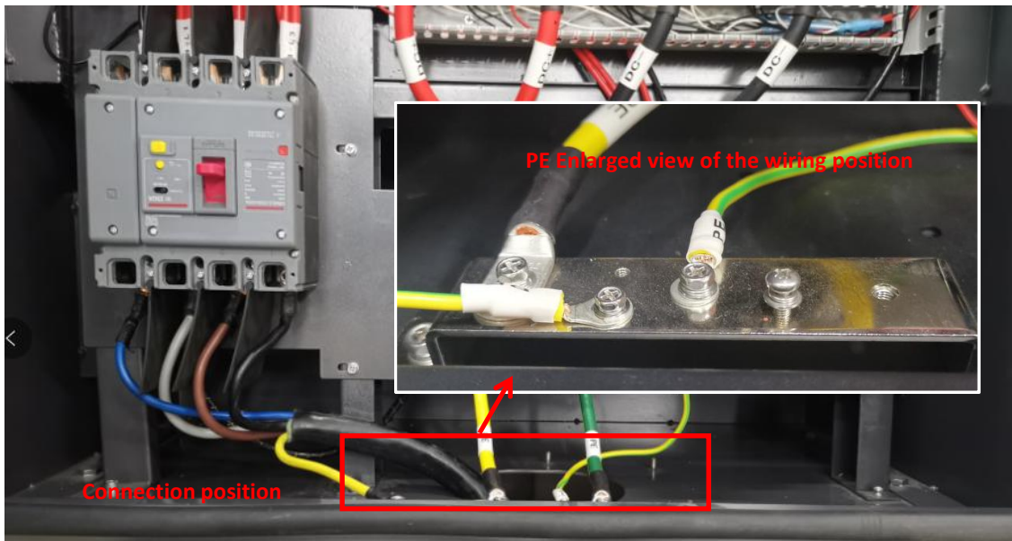
PE position (the bottom wiring position is enlarged as shown on the right)
